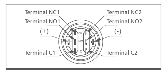
Single & Bi-color
