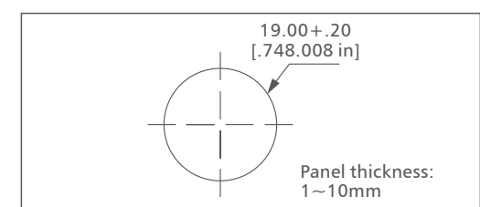
Panel Cutout
