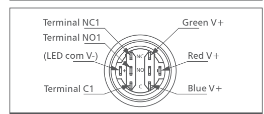
Tri-color
