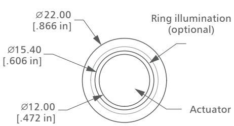
Panel thickness:1~10mm
